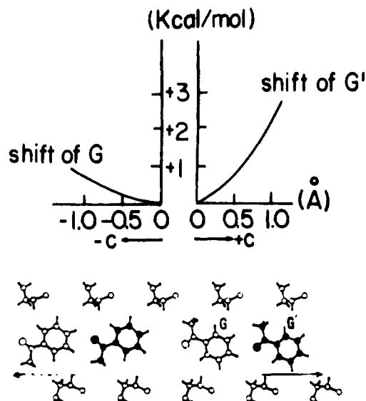
Figure 10. Variation in lattice energy as a result of moving the acetophenone molecules G' and G separately, along the +c and -c directions respectively.
