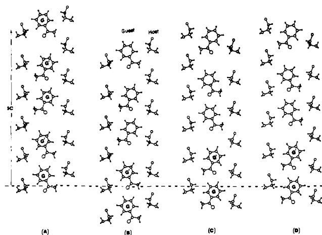
Figure 7. Four disordered guest arrangements in a given channel which differ in their z coordinates. The host-guest contacts are the same for all arrangements.
