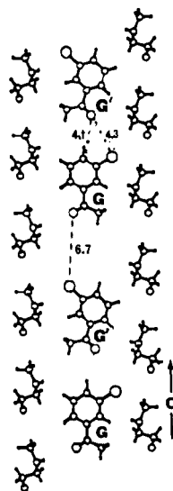
Figure 15. Deduced packing arrangement of chloroacetophenone molecules in the channel viewed perpendicular to the plane of the guest molecule.
