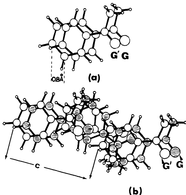
Figure 4. (a) Overlapping pair of guest acetophenone molecules G(x,y,z) and G'(x,y,z') referred to the same molecular site. (b) Molecular overlap of acetophenone guest molecules G (shaded atoms) and G' (unshaded atoms) in the channel. The arrangement may be derived from the molecular pair in (a) by applying 2_1 symmetry to G and G' along the channel.
