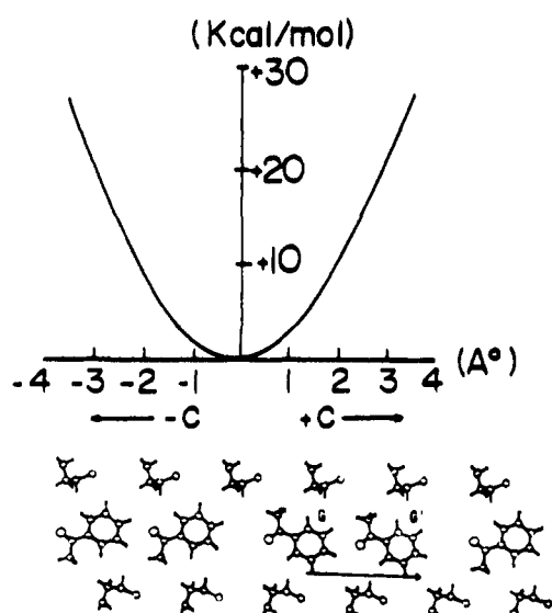
Figure 9. Variation in lattice energy as a result of moving the X-ray-derived chain of acetophenone molecules as a unit along the channel axis.
