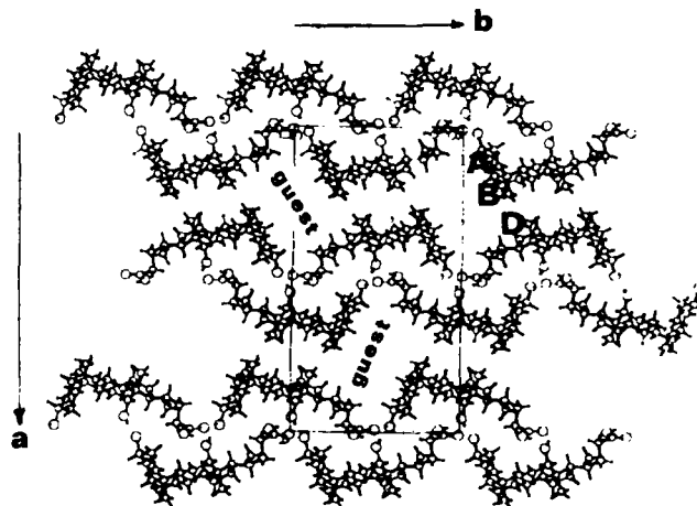
Figure 3. Packing arrangement of DCA molecules in the \alpha motif viewed along the channel c axis. The guest molecules are not shown.
