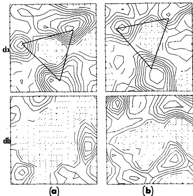
Figure 12. Neutron study of DCA- C_6H_5COCD_3 . Difference density syntheses using calculated structure factors based on contribution of DCA- C_6H_5COC . The four maps were calculated in planes perpendicular to the C7—C8 (i.e., C— CD_3 ) and C7—O (i.e., C=O) bonds of guests G and G'. Each plane passes through a point which lies on extension of bond at a distance 1.1 \text{ \AA} \sin(110-90)^\circ from atom C8 or O1. (a) Molecule G. (b) Molecule G'. (i) Maps perpendicular to the C7—C8 bond. The three peaks of each map correspond to a symmetric D_3 methyl group as demonstrated by the good fit to the triangles of sides 1.8 \text{ \AA} which is the intramolecular distance between D atoms of a methyl group. (ii) Maps perpendicular to the C7—O1 bond. Neither map shows evidence of a D_3 group.
