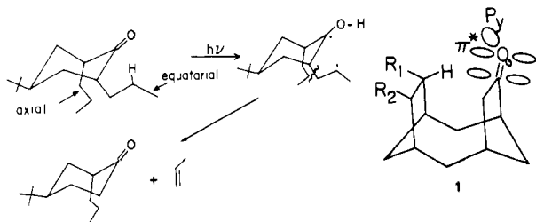
Scheme III
