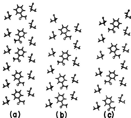
Figure 8. Three guest arrangements for which intermolecular potential energies were calculated: (a) 4:10 guest-host arrangement derived from the X-ray study; (b) 3:8 guest-host arrangement; (c) 1:3 guest-host arrangement.
